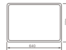
定型压制烘盘 材质：不锈钢、防锈铝合金 Shaped Pressed Baking-Plate Material:stainless steel,rustproof aluminium alloy
