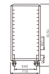
手工井字网盘 Manual multi-square mesh plate
